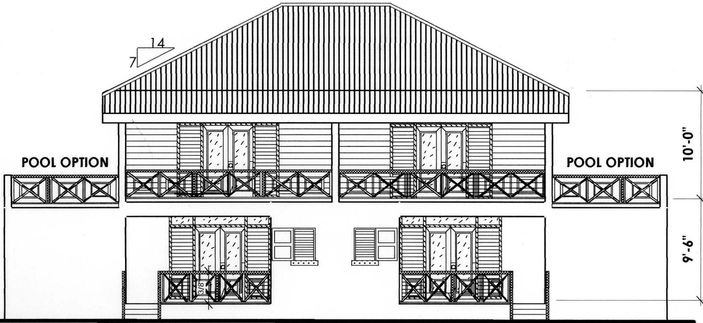
FRONT ELEVATION
