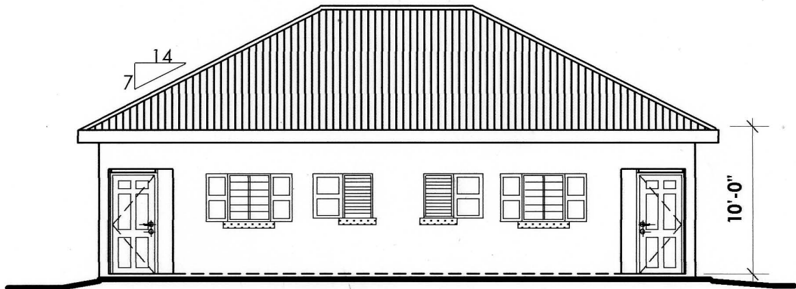
ENTRANCE ELEVATION
